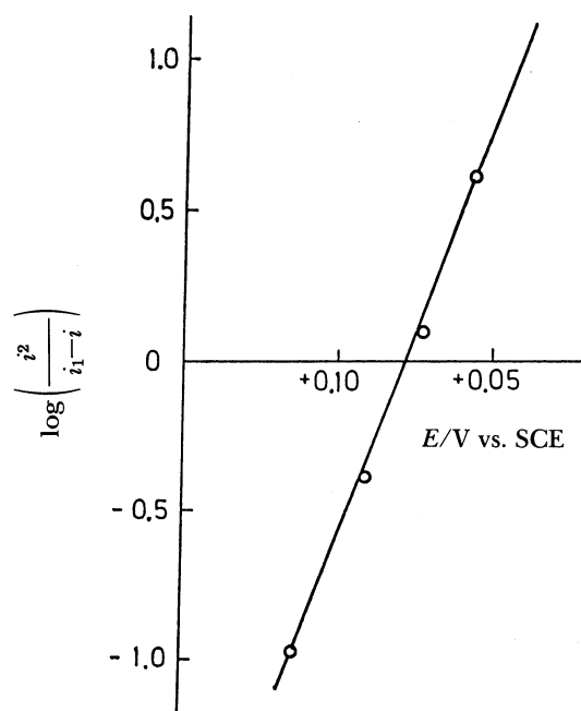
Fig. 4. \log(i^2/(i_l - i)) against E plot: Ag(II)-[14]aneN 4 complex; 0.40 mM, pH=4.90, [OAc^-]=0.050 M, [SO_4^{2-}]=0.20 M, 25 °C.
